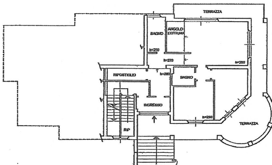
PIANO TERRENO
